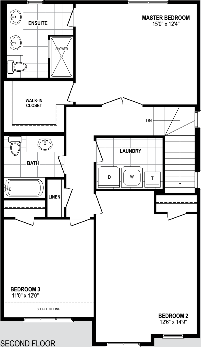
SECOND FLOOR ELEV. B
