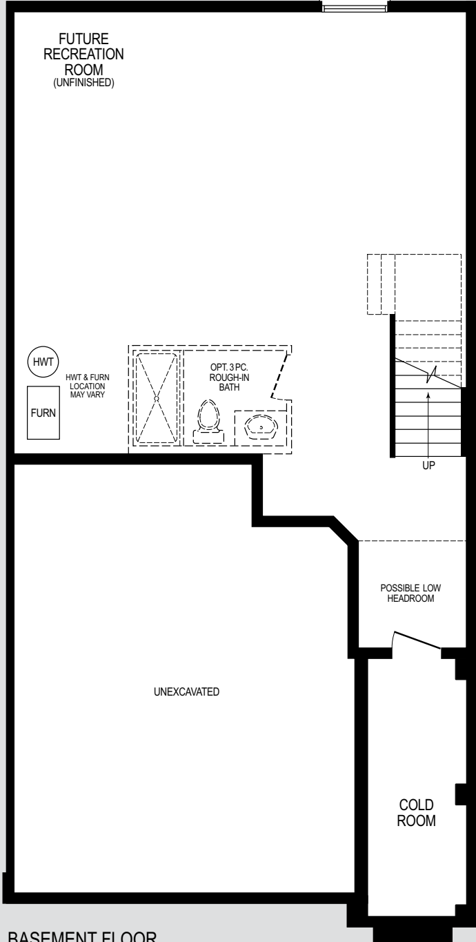
BASEMENT FLOOR ELEV. B
