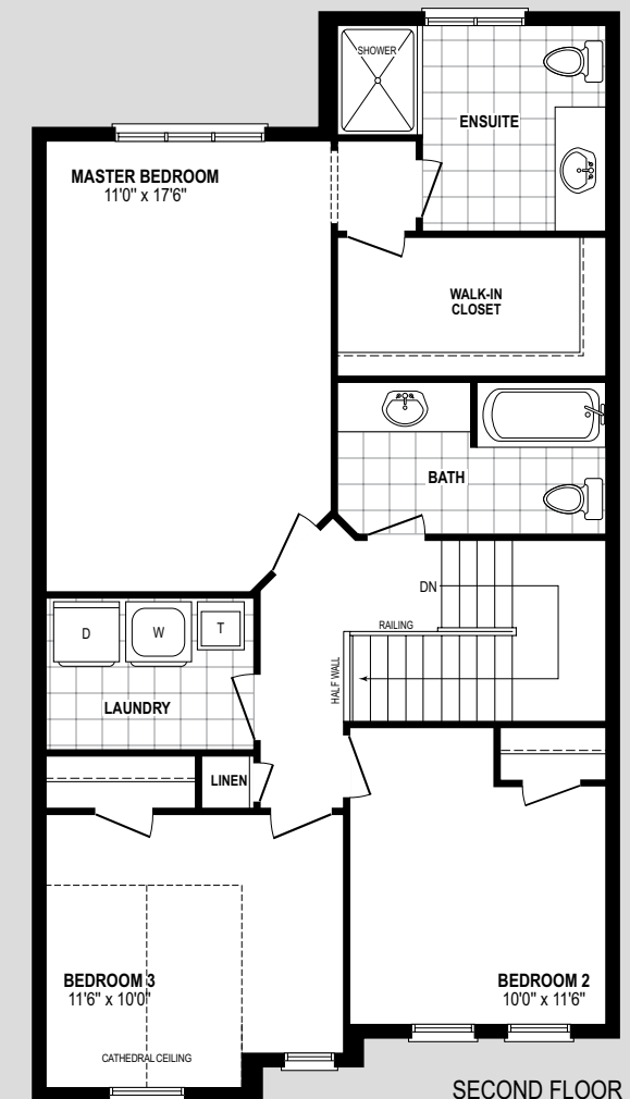
SECOND FLOOR ELEV. C
