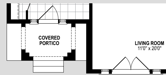
GROUND FLOOR ELEV. B
