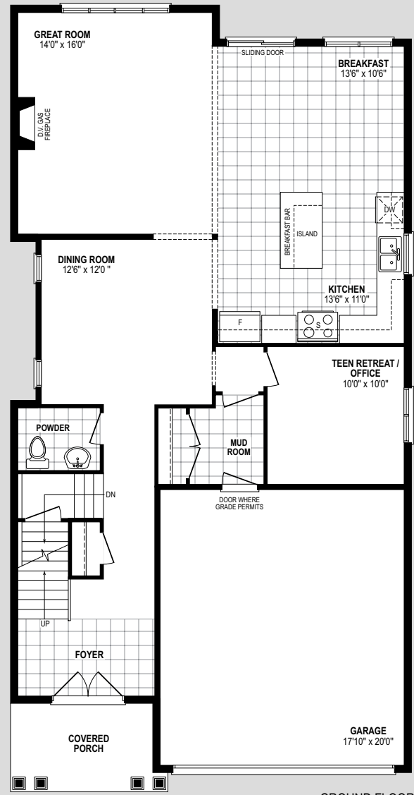
GROUND FLOOR ELEV. C
