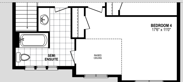
SECOND FLOOR ELEV. B
