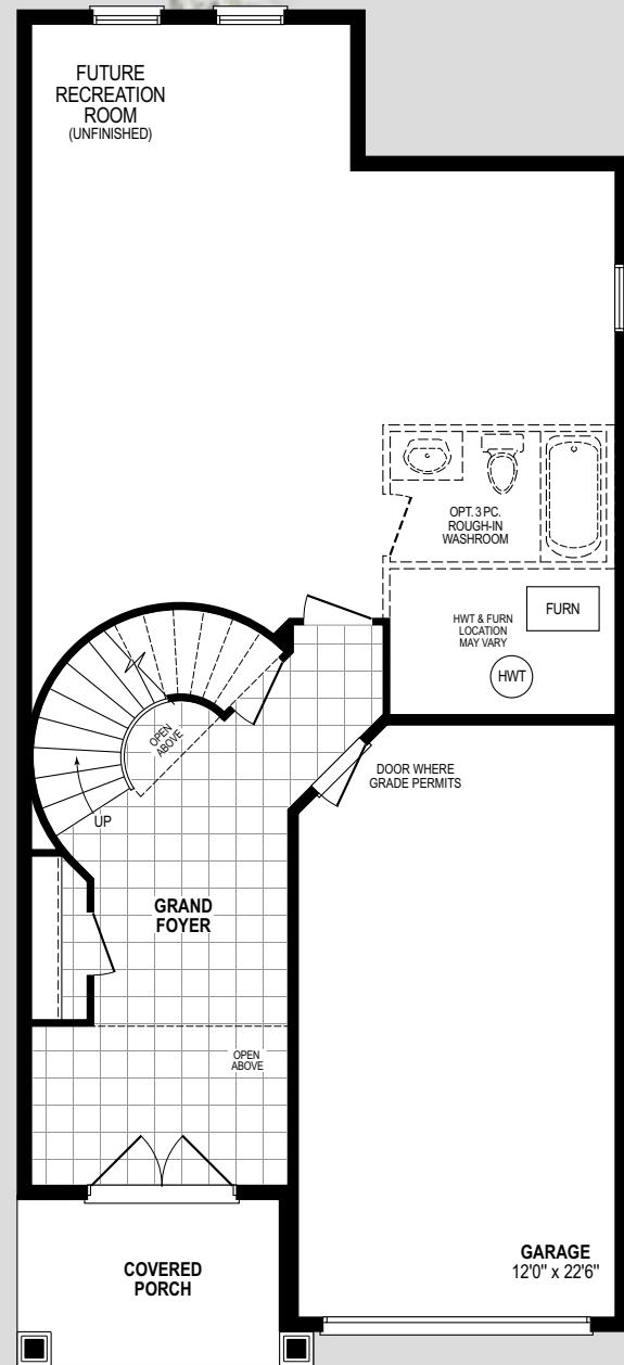
BASEMENT FLOOR ELEV. C
