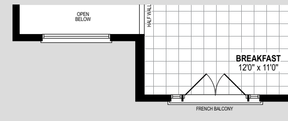
GROUND FLOOR ELEV. B
