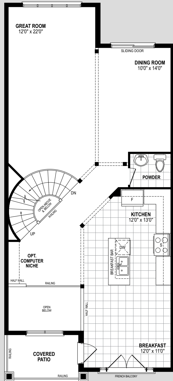
GROUND FLOOR ELEV. C
